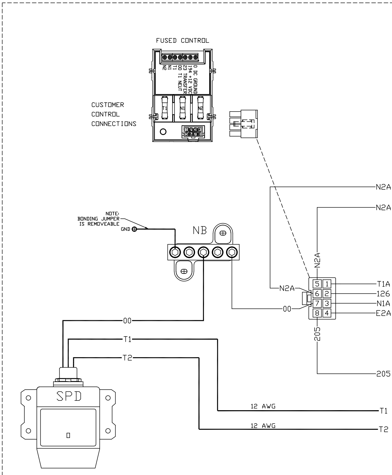
WIRING - DIAGRAM
